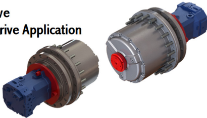
O&K Drive Capstan Winch Application
