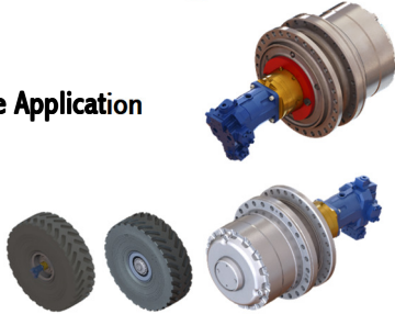
O&K Drive Wheel Drive Application
