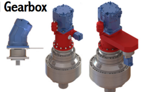
Black Bruin Motor Integrated Single Stage Planetary Gearbox
