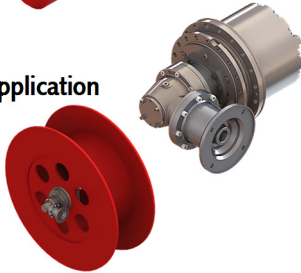
Black Bruin Motor Wheel Drive Application
