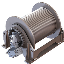
O&K Winch Gearbox Winch Drive Package One Piece Rigid Frame Integrated Valve
